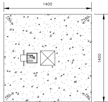
SPLASH PAD— PLAN (scale 1:20)
