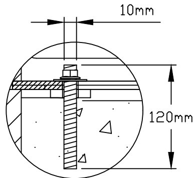
FIXING DETAIL
