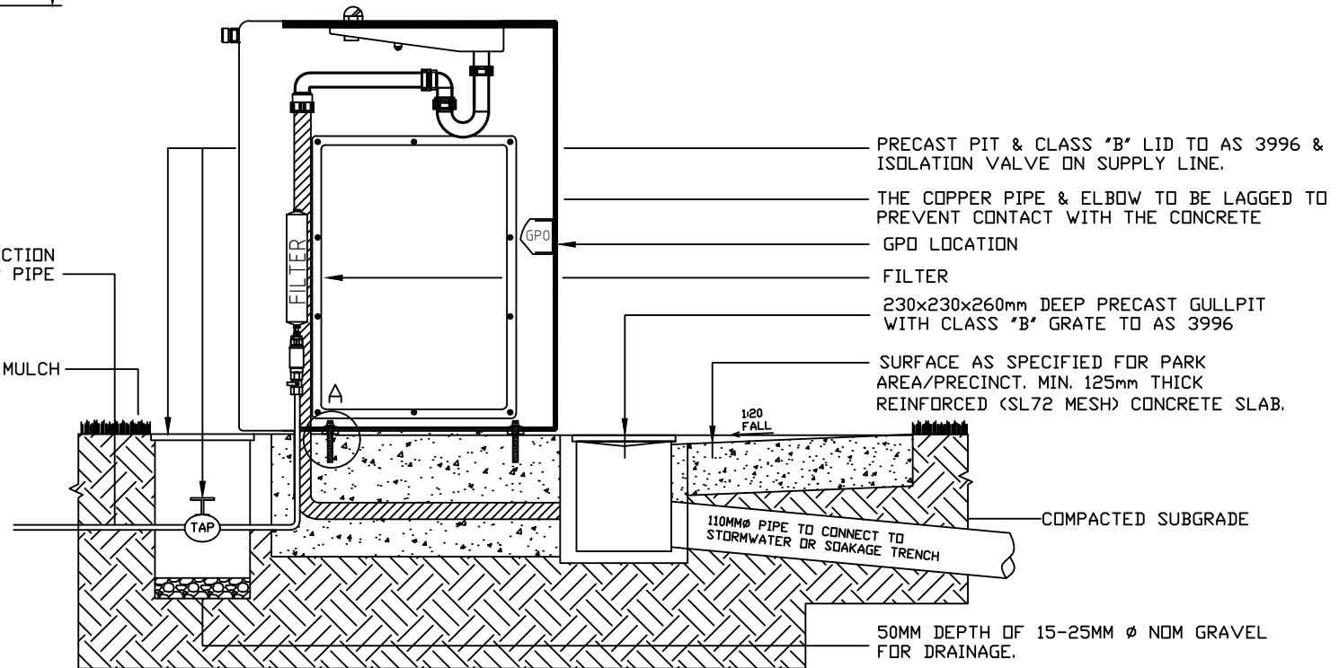
FIXING DETAIL
