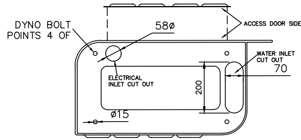
VIEW A
